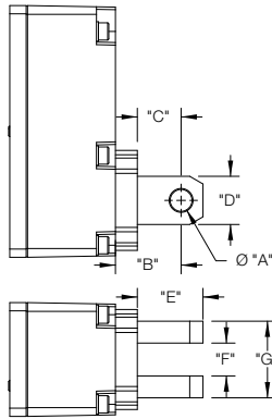
Clevis and Eye Dimensions, Imperial and Metric
