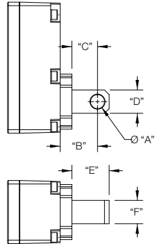
Rear Eye (KSRE-75, KSME-75)
