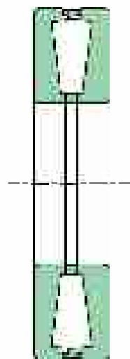
Tapered Thrust T-16050 8" x 16.5" x 3.625" Dynamic Capacity = 752,120 lbs
