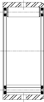
Outer Ring and Roller Assembly B-XXX
