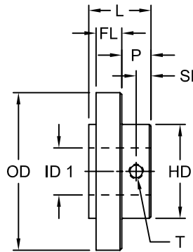
S Type Flange
