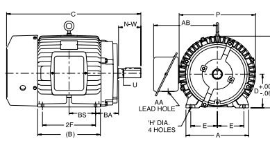
Typical Rigid Base Motor
